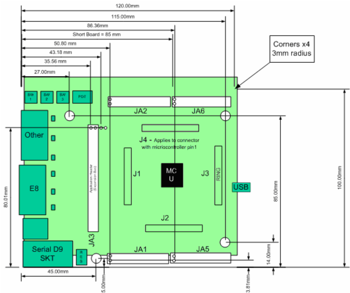
Figure 4.2 : Board Dimensions
