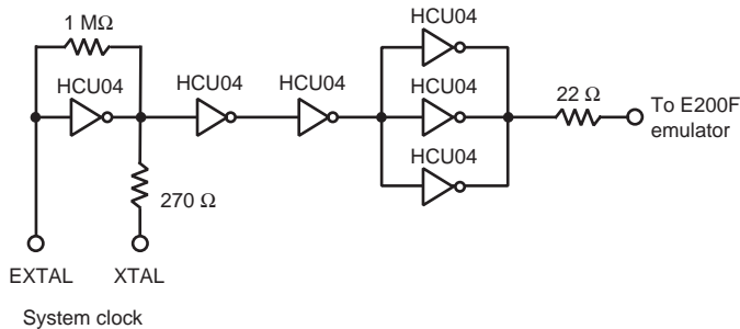
Figure 8 Clock Oscillator
