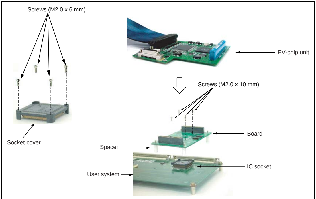
Figure 1 User System Interface Board for the SH7146 PLQP0080JA-A (Former Code: FP-80WV) Package
