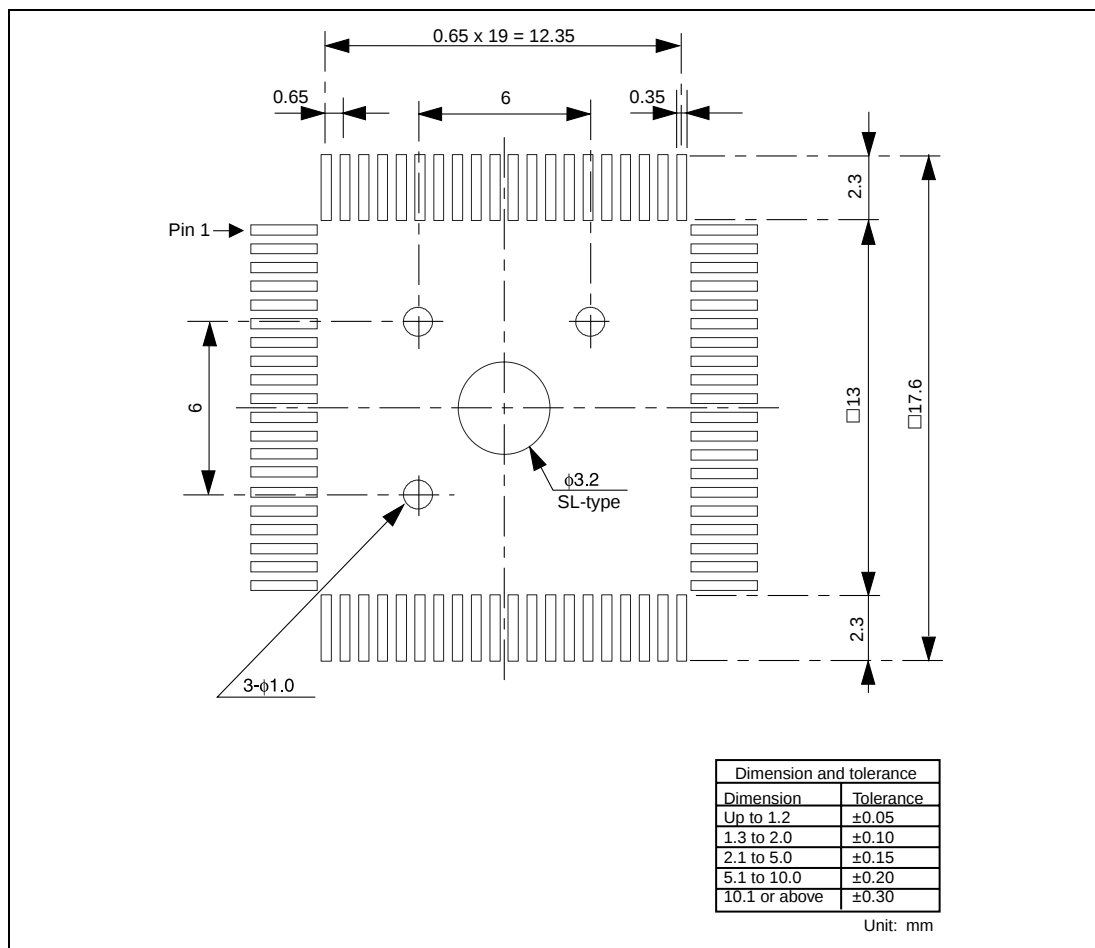
Figure 4 Recommended Dimensions for Mount Pad
