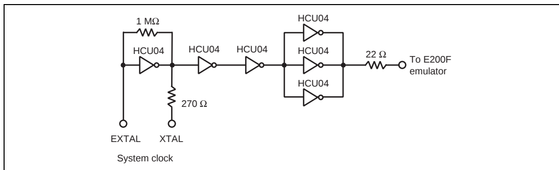
Figure 8 Clock Oscillator
