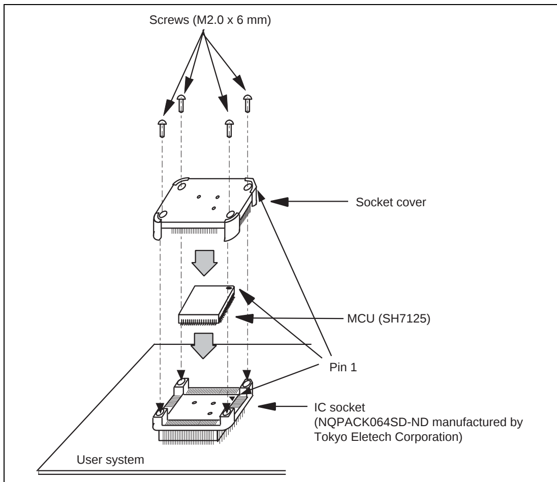
Figure 7 Installing MCU to User System
