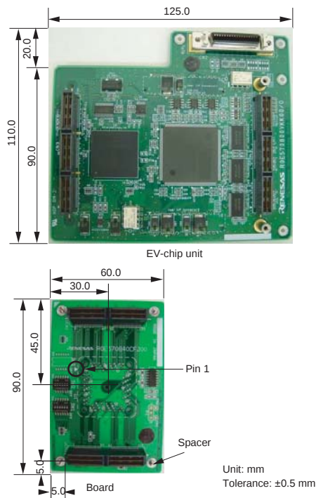
Figure 5 Dimensions for EV-Chip Unit and User System Interface Board
