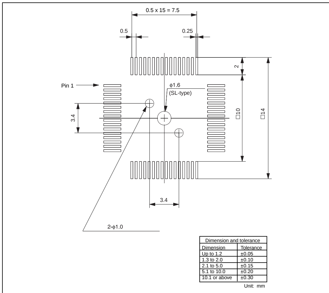
Figure 4 Recommended Dimensions for Mount Pad
