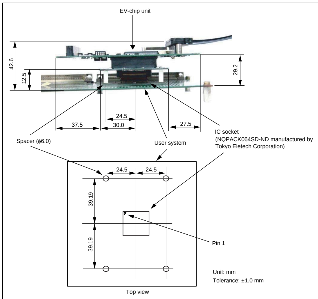
Figure 6 Resulting Dimensions after Connecting User System Interface Board (when Connecting EV-Chip Unit)
