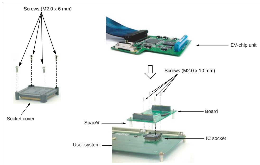
Figure 1 User System Interface Board for the SH7086 PLQP0176KB-A (Former Code: FP-176EV) Package
