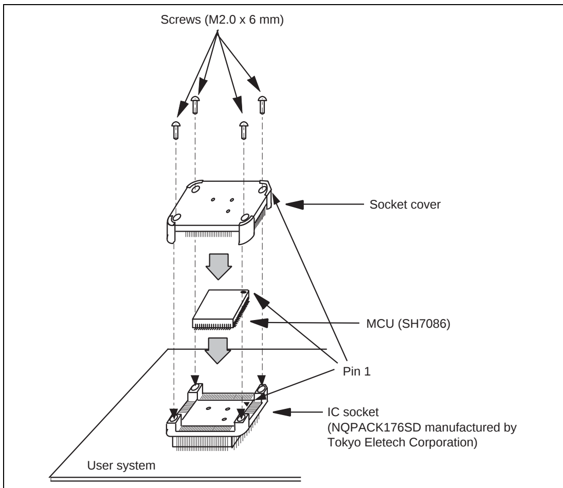
Figure 11 Installing MCU to User System
