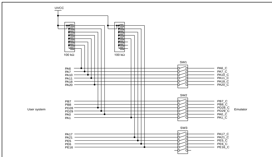
Figure 3 Circuit for Masking Signals
