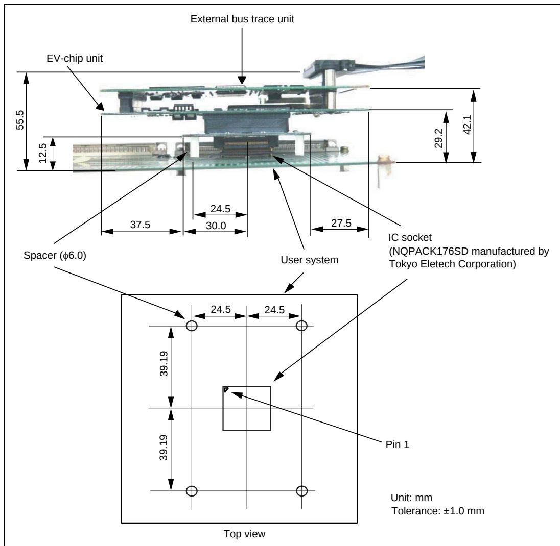
Figure 9 Resulting Dimensions after Connecting User System Interface Board (when Connecting External Bus Trace Unit and EV-Chip Unit)
