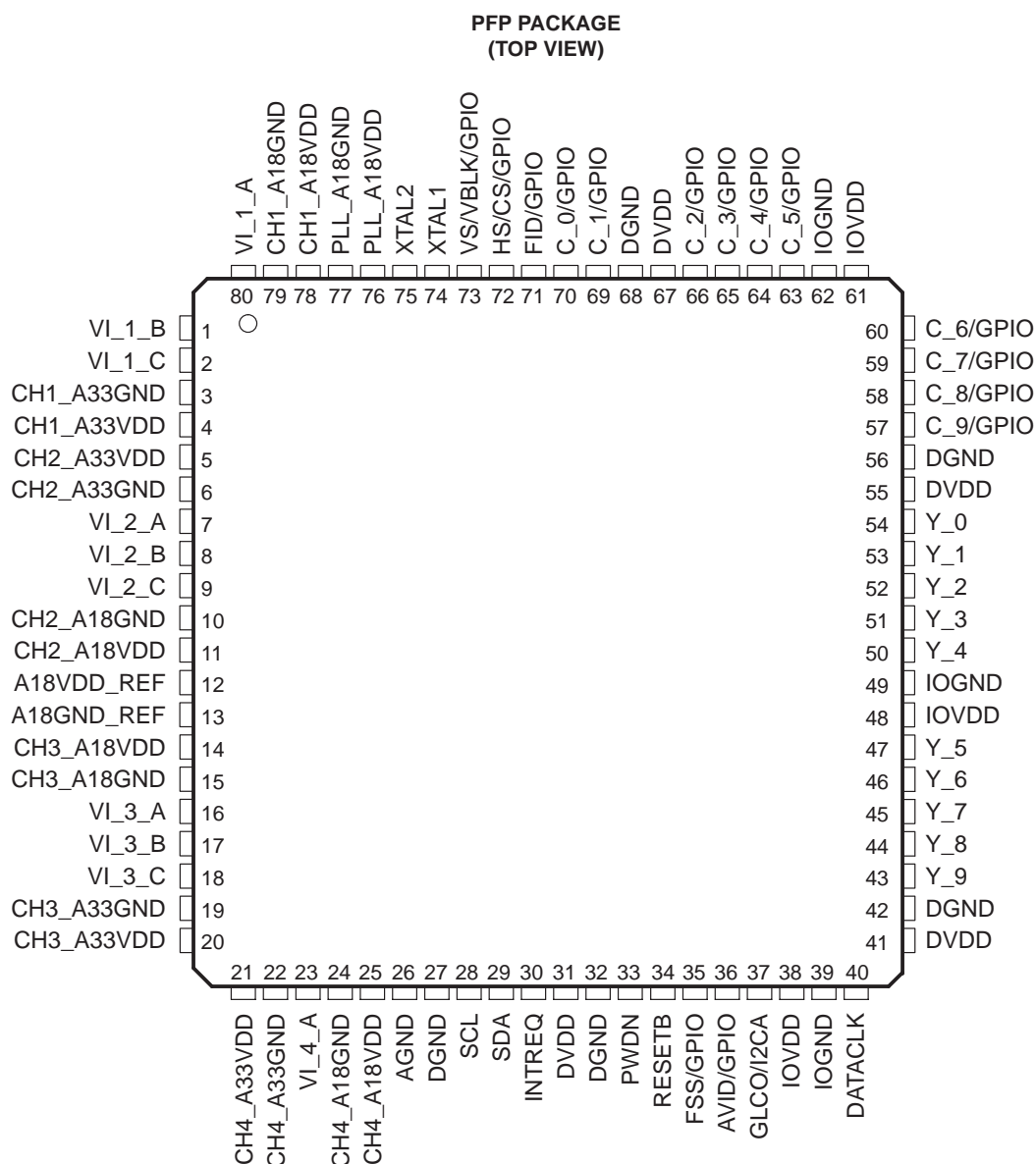
Figure 1–2. Terminal Assignments
