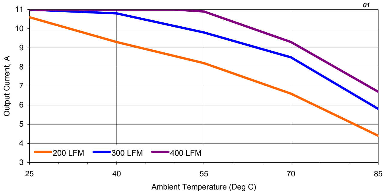
Figure 5. QBC11ZH-T Derating Curves
