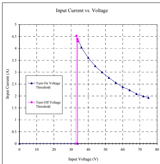
Figure 2. QBC11ZH-T Input Characteristics
