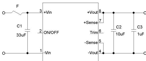
Figure 3. Typical Application of QBC11ZH-T
