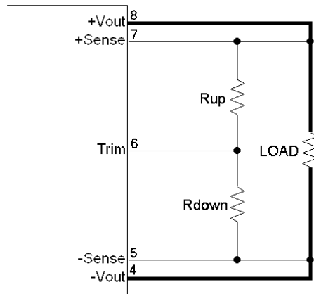
Figure 4. QBC11ZH-T Trim Schematic
