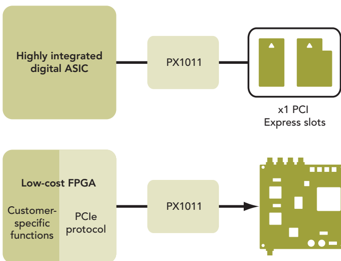
The PX1011 provides digital ASICs and low-cost FPGAs with mixed-signal PHY functionality
