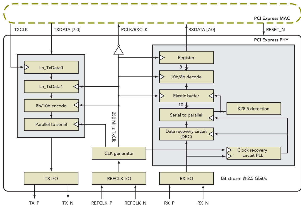
PX1011 block diagram
