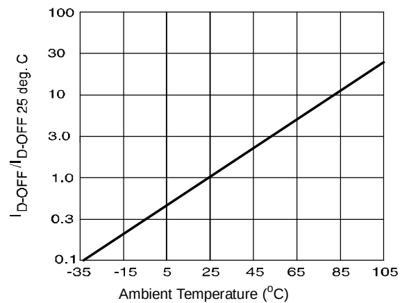
Figure 4. Typical Normalized Off-State Leakage
