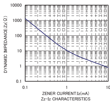
Zz-Iz CHARACTERISTICS
