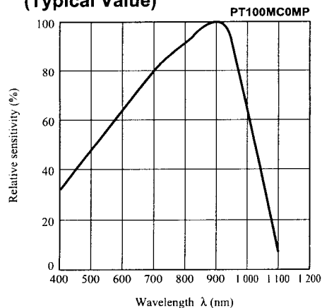
Fig.9 Relative Sensitivity vs. Wavelength (Typical Value)
