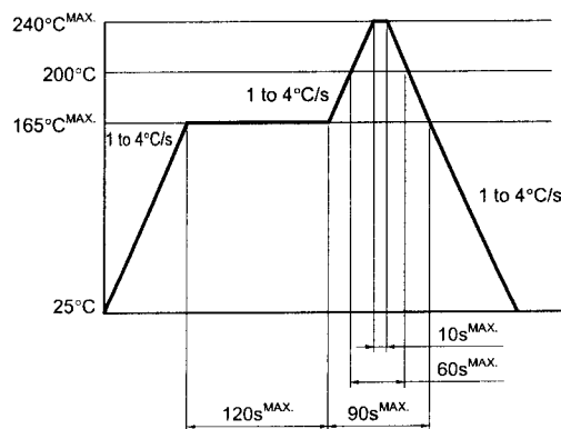
Fig.15 Reflow Soldering
