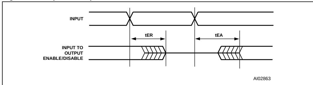
Figure 37. Input to Output Disable / Enable
