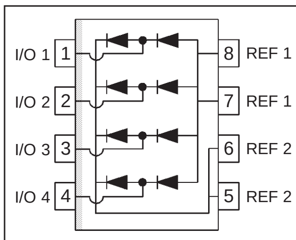
FUNCTIONAL DIAGRAM : DA112S1
