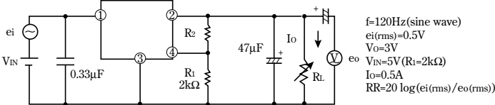
Fig. 2 Test circuit for Ripple Rejection
