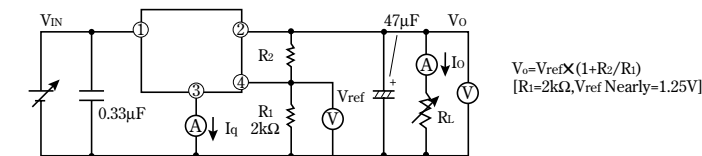
Fig. 1 Test Circuit
