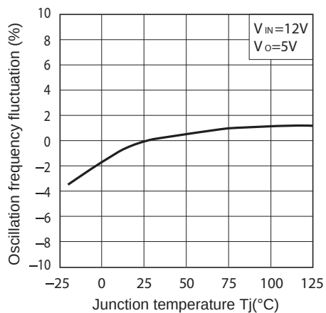
Fig.10 Oscillation Frequency Fluctuation vs. Junction Temperature
