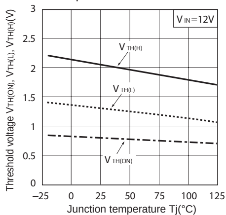
Fig.12 Threshold Voltage vs. Junction Temperature
