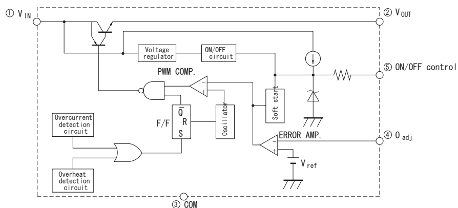
Fig.14 Block Diagram
