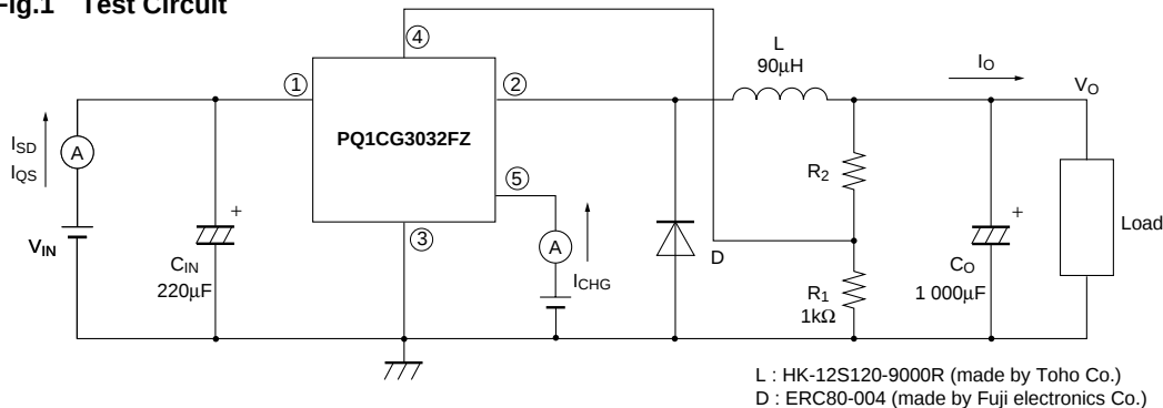
Fig.1 Test Circuit
