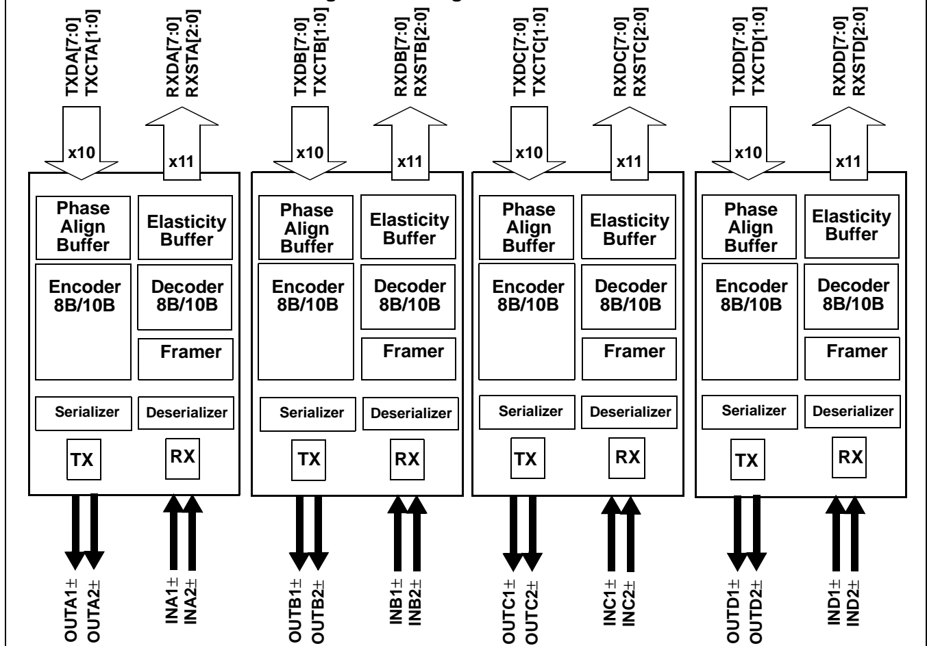
CYP15G0401DXB Transceiver Logic Block Diagram
