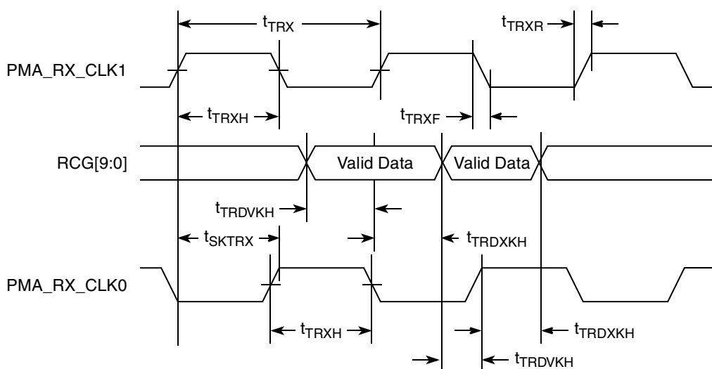
Figure 20. TBI Receive AC Timing Diagram
