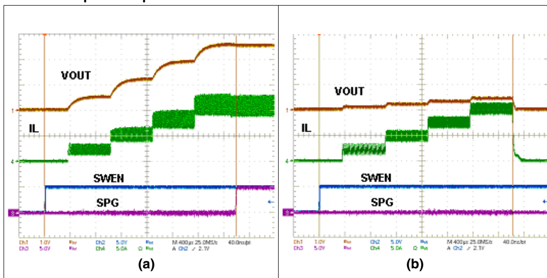
Figure 32. Soft-start at heavy load (a) and short-circuit (b) condition, pulse-skip enabled
