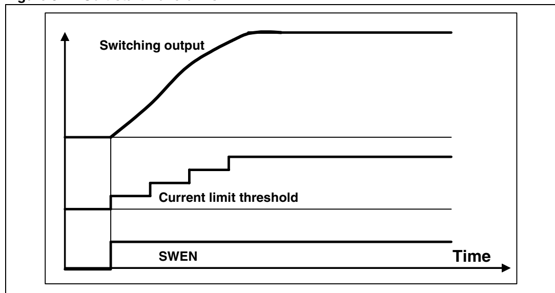
Figure 31. Soft-start waveforms
