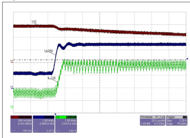
Figure 25. Output OV (1V5) @ R_{CSNS} = 1\text{ M}\Omega
