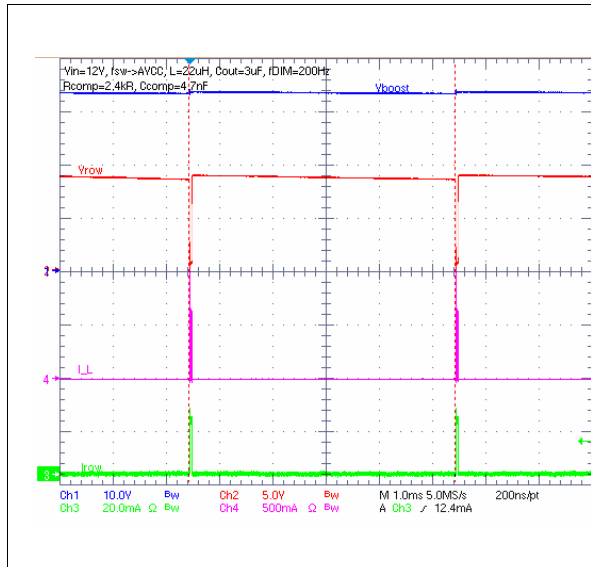
Figure 23. Working waveforms @ f_{DIM} = 200 \text{ Hz} , D = 50 \%
