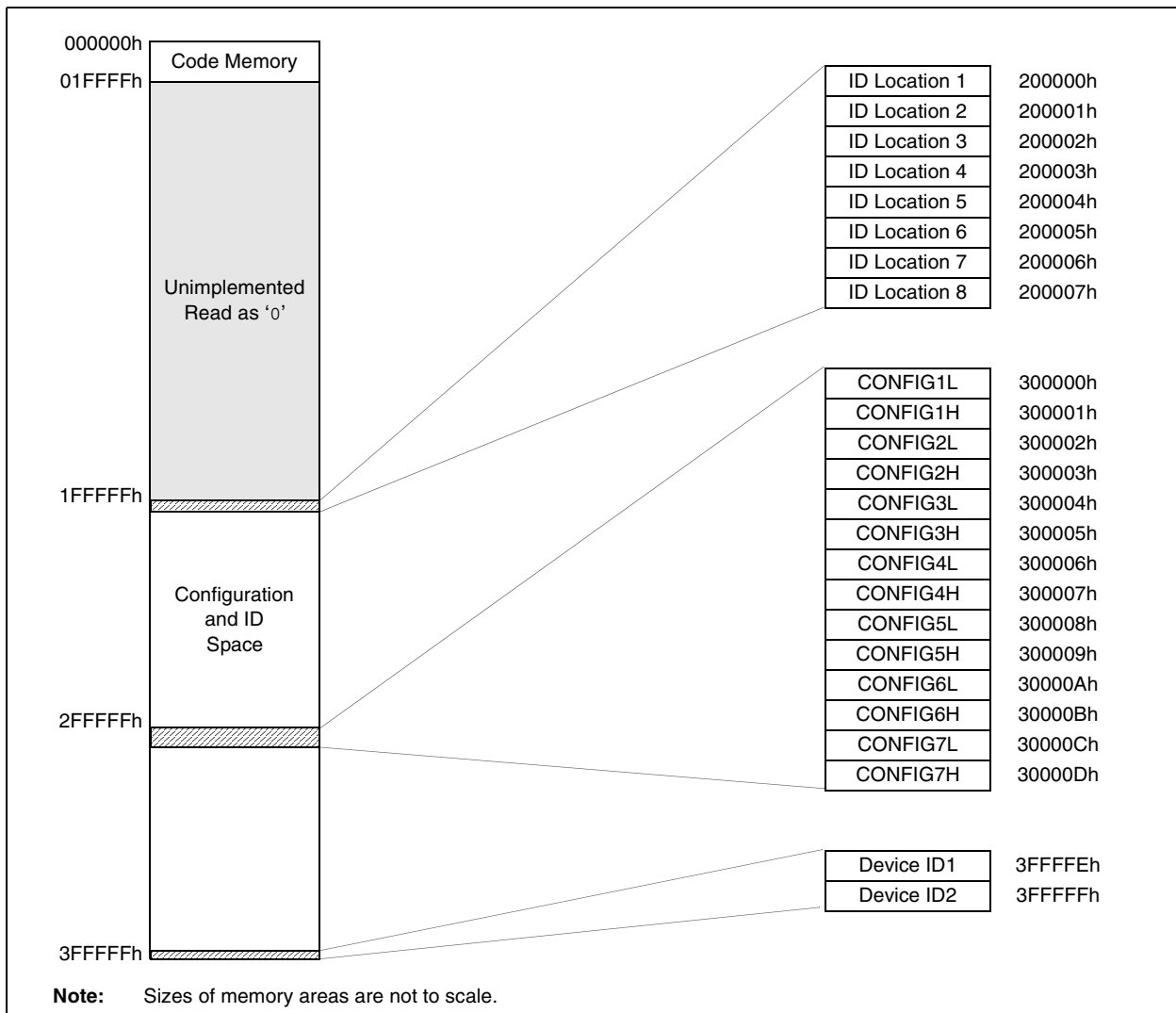
FIGURE 2-9: CONFIGURATION AND ID LOCATIONS FOR PIC18F2XX0/2X21/2XX2/2XX5/4XX0/4X21/4XX2/4XX5 DEVICES
