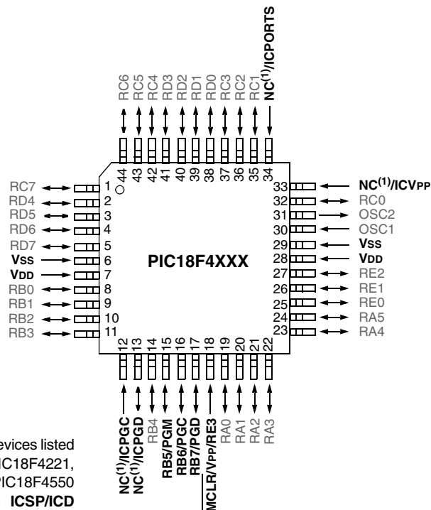
FIGURE 2-2: PIC18F2XX0/2X21/2XX2/2XX5/4XX0/4X21/4XX2/4XX5 FAMILY PIN DIAGRAMS
