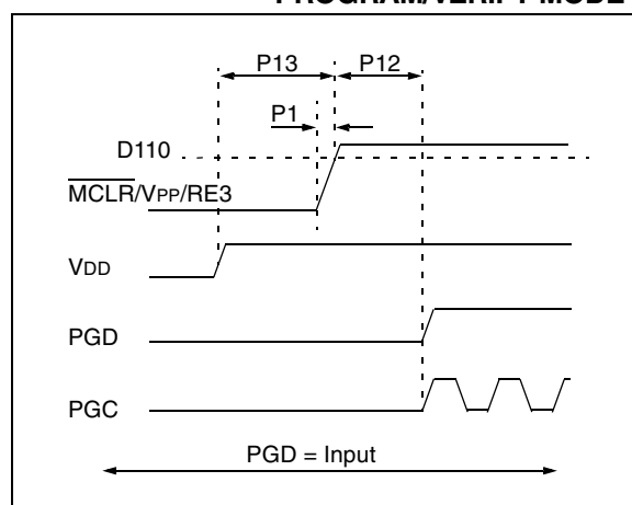
FIGURE 2-11: ENTERING HIGH-VOLTAGE PROGRAM/VERIFY MODE
