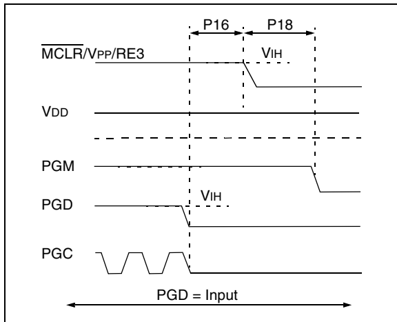
FIGURE 2-14: EXITING LOW-VOLTAGE PROGRAM/VERIFY MODE
