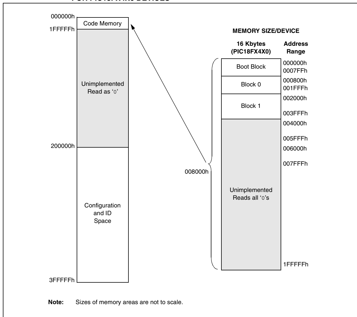
FIGURE 2-6: MEMORY MAP AND THE CODE MEMORY SPACE FOR PIC18FX4X0 DEVICES
