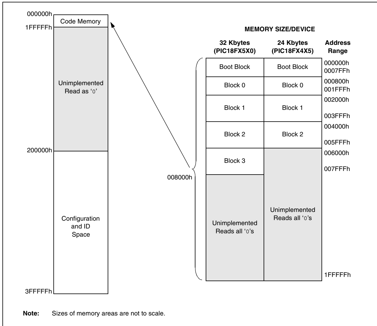
FIGURE 2-5: MEMORY MAP AND THE CODE MEMORY SPACE FOR PIC18FX4X5/X5X0 DEVICES
