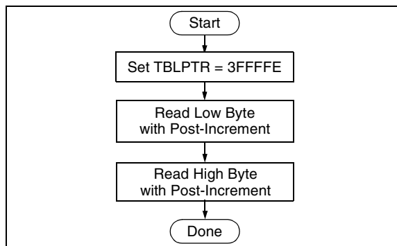
FIGURE 5-1: READ DEVICE ID WORD FLOW
