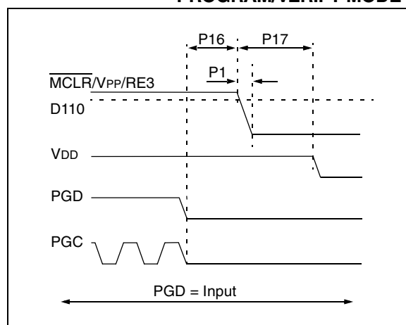
FIGURE 2-12: EXITING HIGH-VOLTAGE PROGRAM/VERIFY MODE
