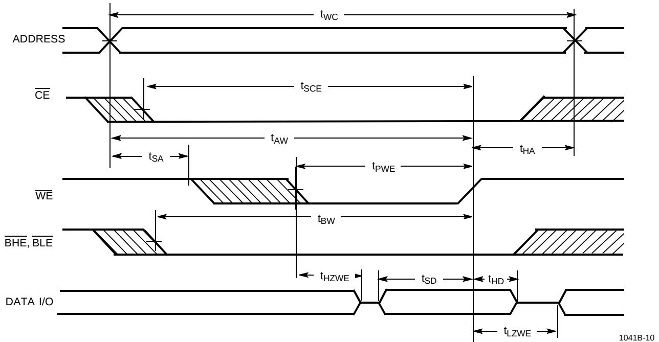
Write Cycle No. 3 ( \overline{\text{WE}} Controlled, \overline{\text{OE}} )
