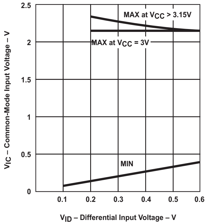
Figure 2. Common-Mode Input Voltage vs. Differential Voltage
