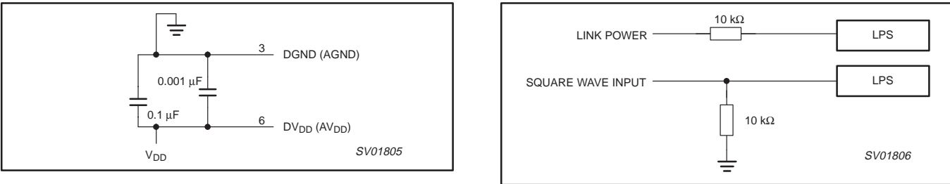
Figure 7. Non-isolated connection variations for LPS
