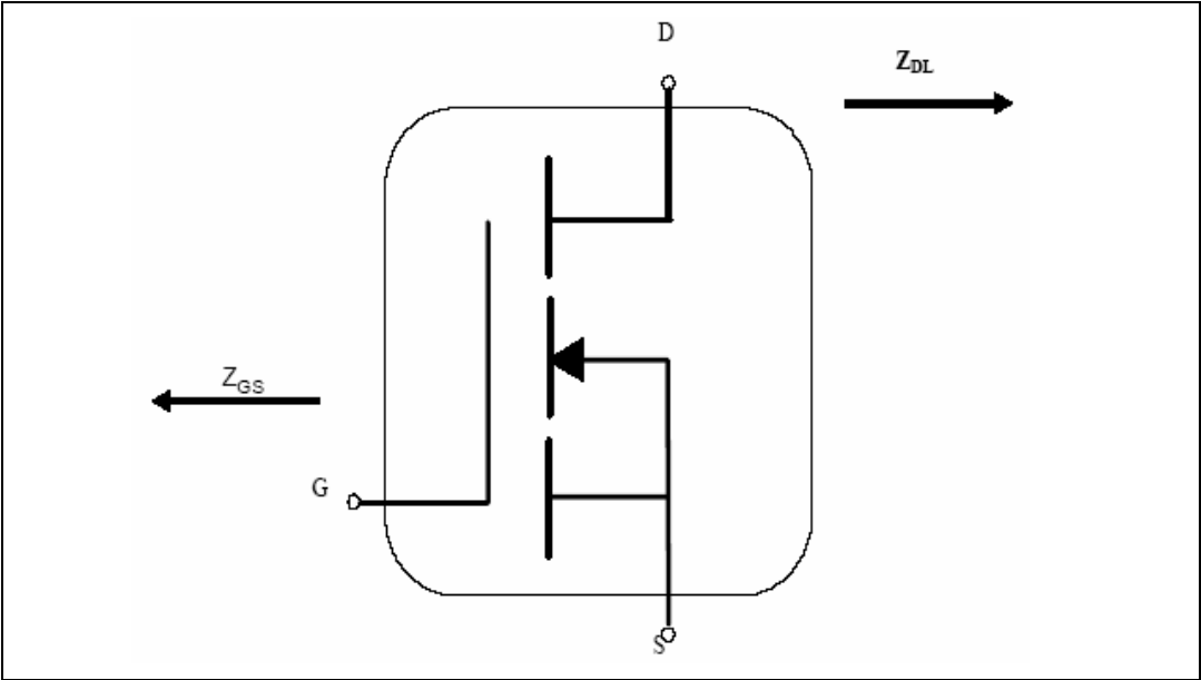
Figure 3. Impedances
